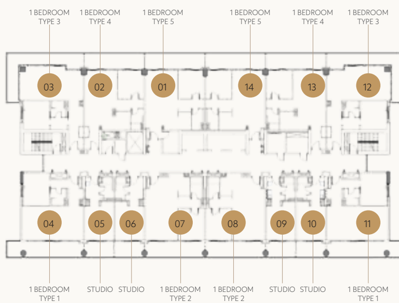
LEVELS 02-03
