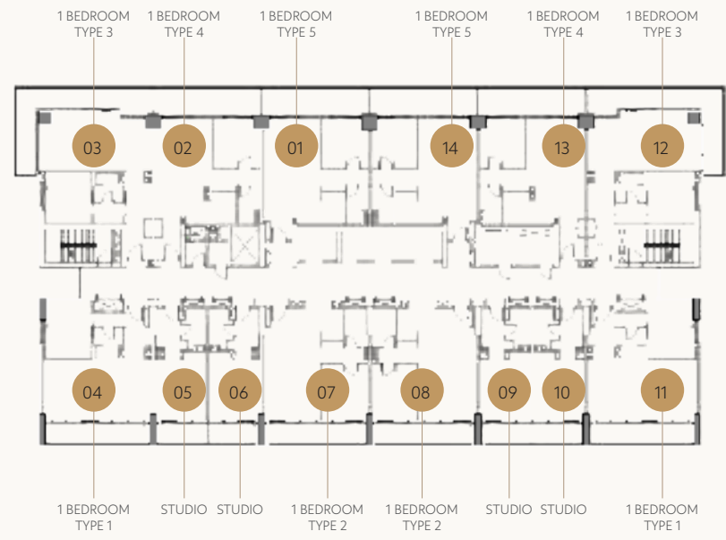
LEVELS 02-03
