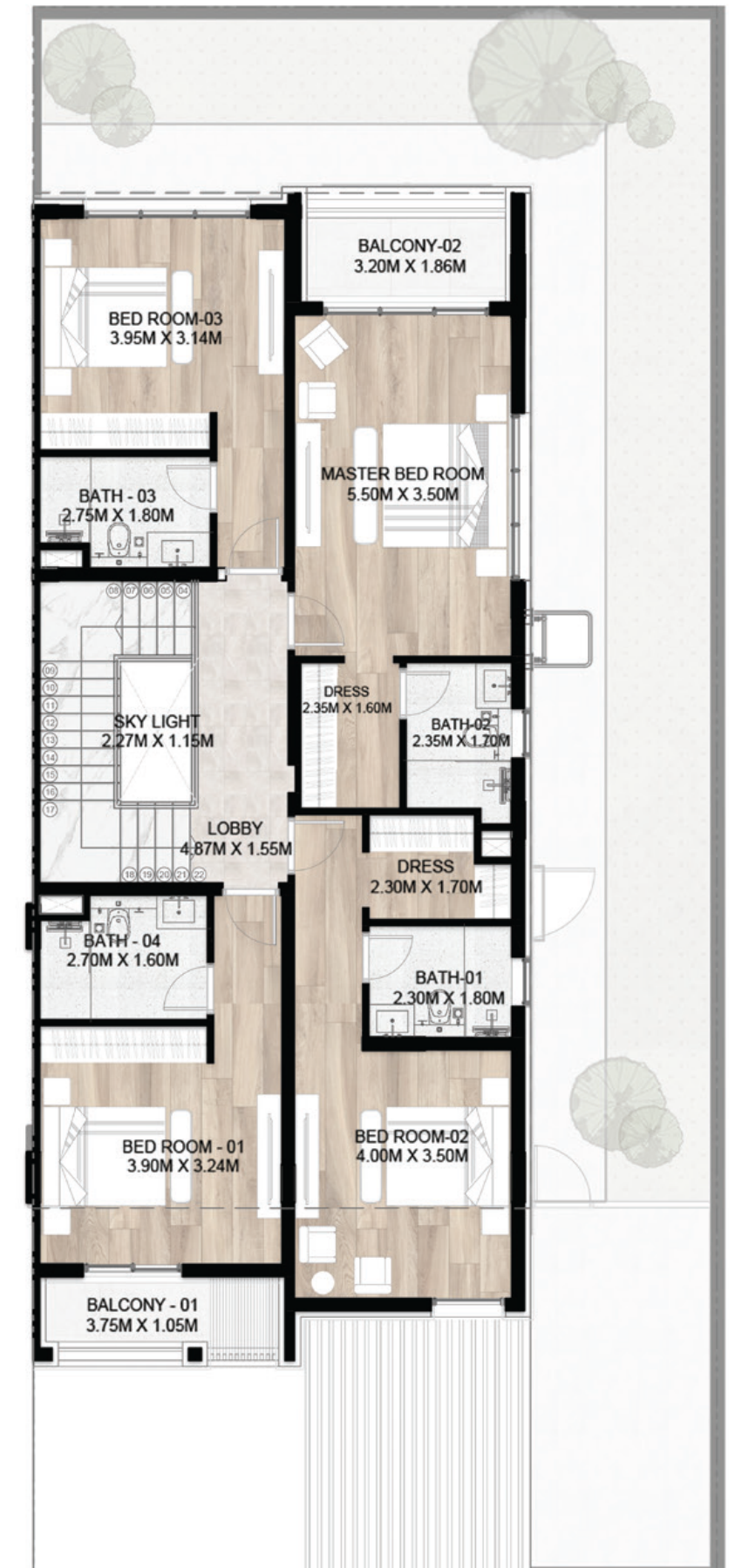
First floor
